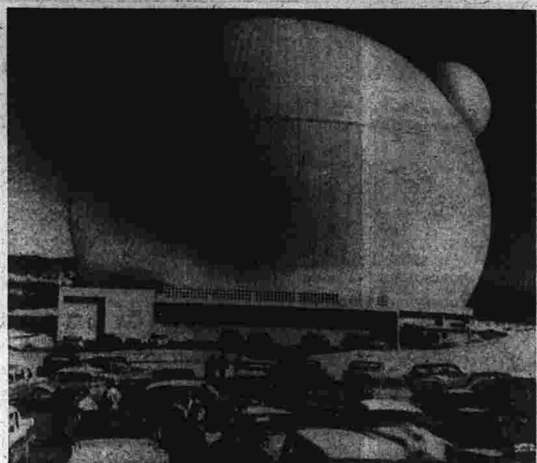
Cars of visitors crowd parking lot beside Bell Telephone Laboratories satellite communication station. Bubble, 160 feet high, houses 300-ton "ear" to pick up signals from orbiting satellites. No. 10, the little bubble, isn't because the engineers blew too hard. It is to fit around equipment inside when balloon is deflated to permit erection of permanent dome. (AP Photofax).
